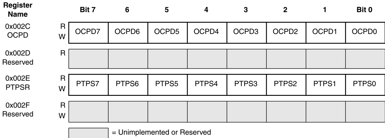
Figure 22-5. TIM16B8CV2 Register Summary (Sheet 3 of 3)
