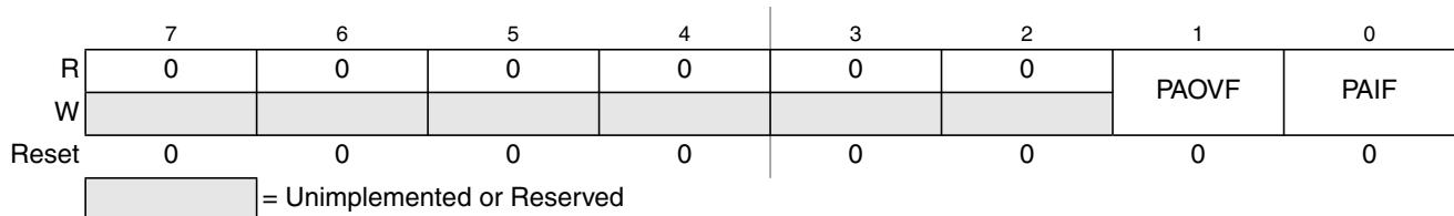
Figure 14-36. Pulse Accumulator A Flag Register (PAFLG)
